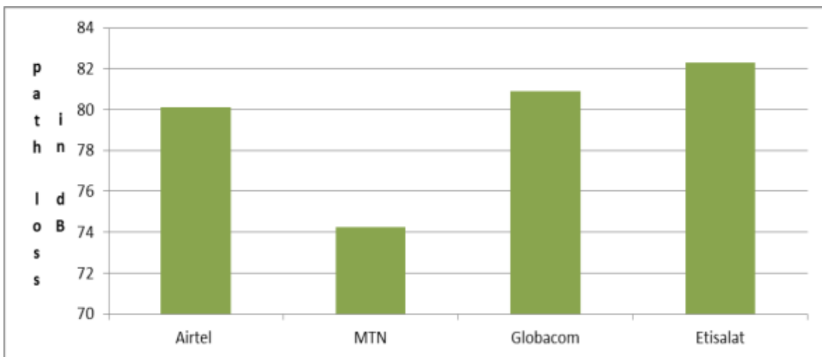
Figure 2: Average measure Propagation Path loss
