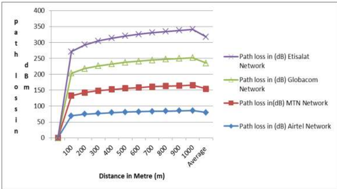
Figure 1: measured path loss against Distance
